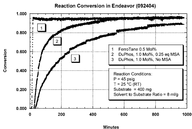
Figure 1. Reactivity of Et-FerroTANE-Rh catalyst vs Et-DuPHOS-Rh catalyst.
